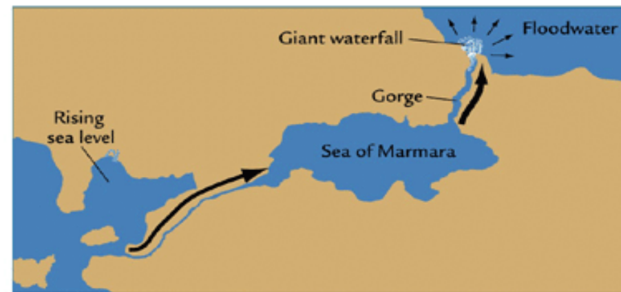
B Deglacial flood (7600 years ago)
